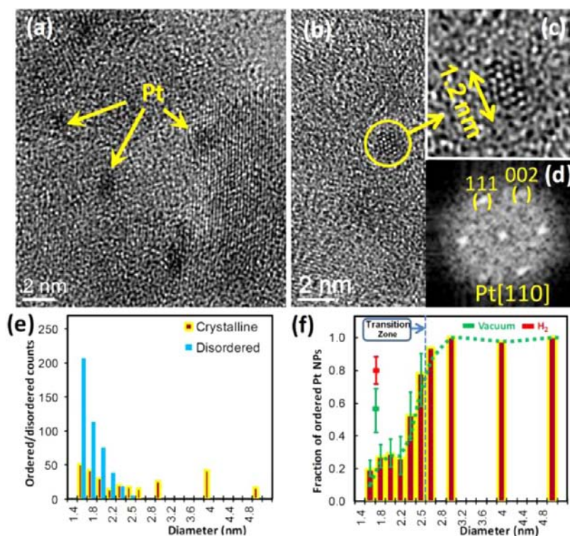
Figure 2. FS-HRTEM images and histograms of Pt NP structures on \gamma -Al 2 O 3 . (a) Disordered 1.2–1.5 nm NPs and (b) ordered 1.2 nm NP, magnified in (c) and its FFT in (d) showing fcc along [110]. (e) Histogram of ordered and disordered NPs. (f) Fraction of ordered NPs vs size, where NPs > 2.5 nm were all observed to be ordered. ETEM data in (f) were collected from many NPs: “vacuum” refers to the as-prepared samples observed in the TEM column, and “H 2 ” refers to ETEM data after annealing 30 min at 385 °C in 1 Torr H 2 in situ and then cooled to room temperature. The error bars reflect the 95% confidence interval in the data.
